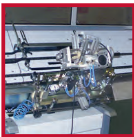
Hangers-former and feeder.
